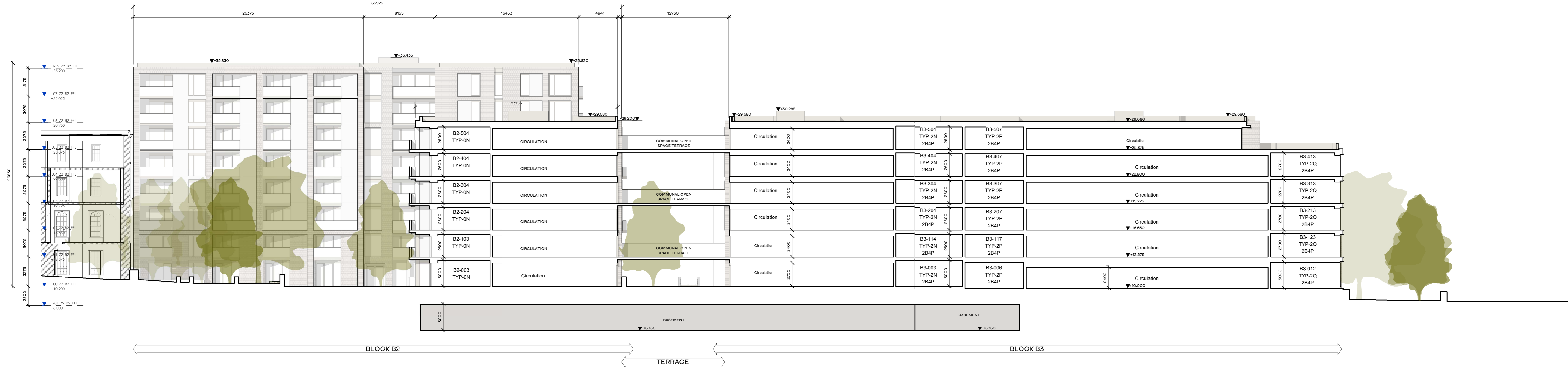
3 GA Section - Section C-C 1:200
