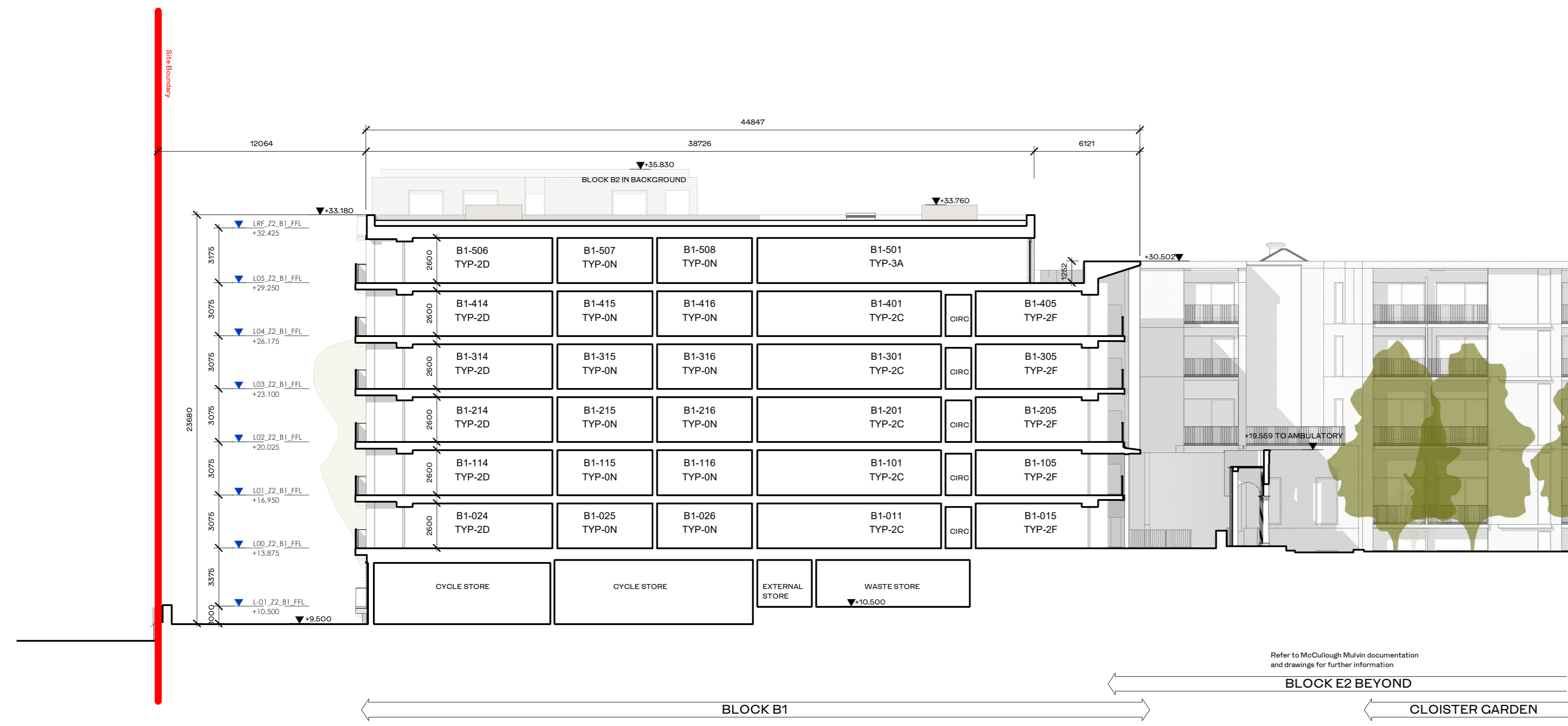
1 GA Section - Section A-A 1:200
